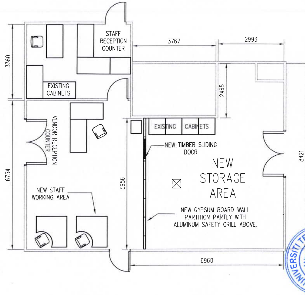
LAYOUT PLAN OF STORE UNIT, UTB ( Room GF.09 )
